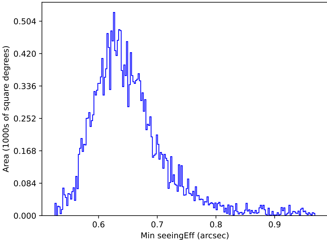
baseline_v3.3_10yrs All sky y band: Min seeingEff
