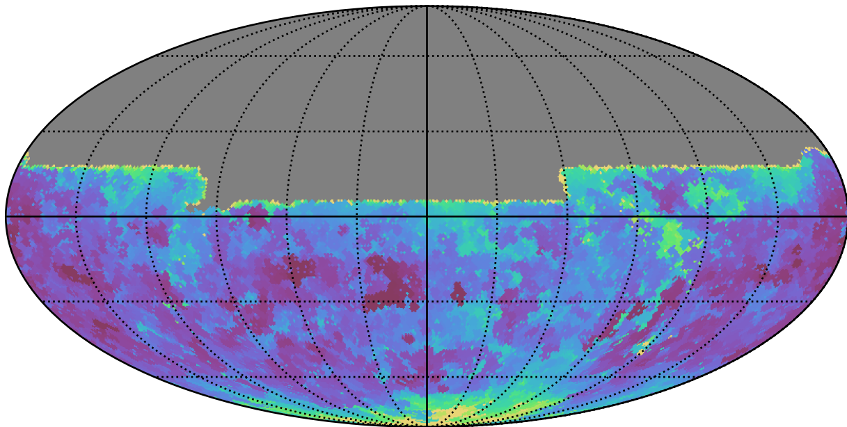
baseline_v3.3_10yrs All sky u band: Min seeingEff
