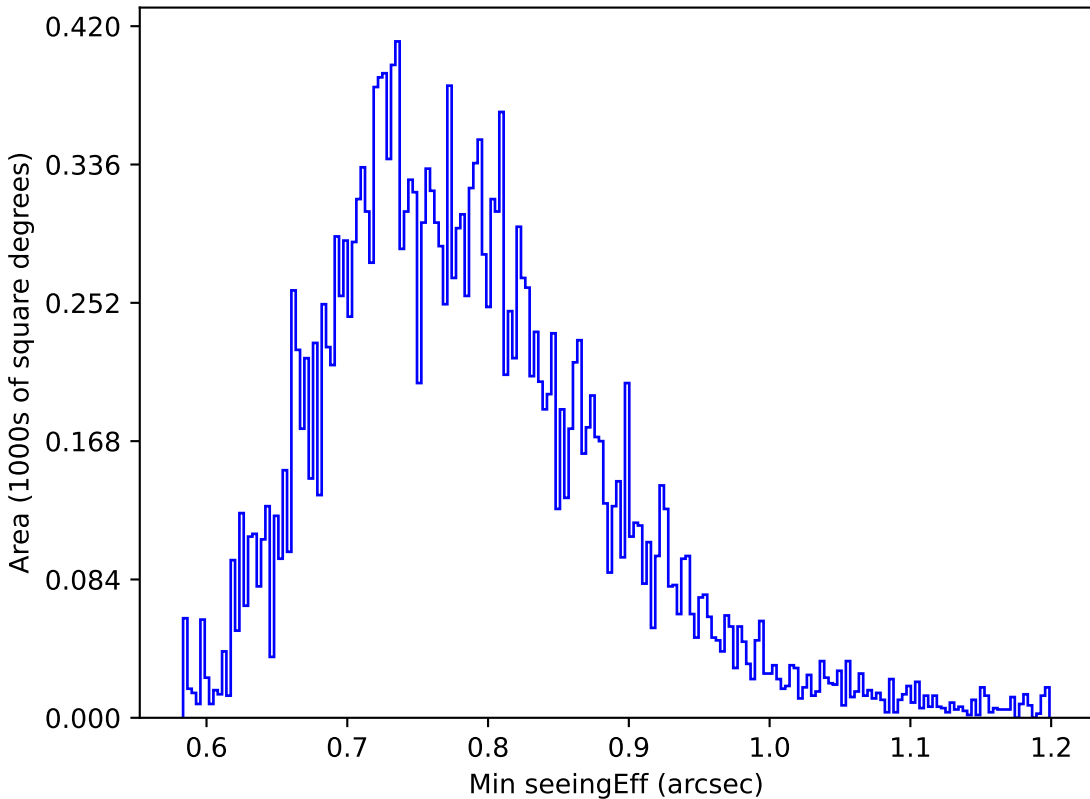
baseline_v3.3_10yrs All sky u band: Min seeingEff
