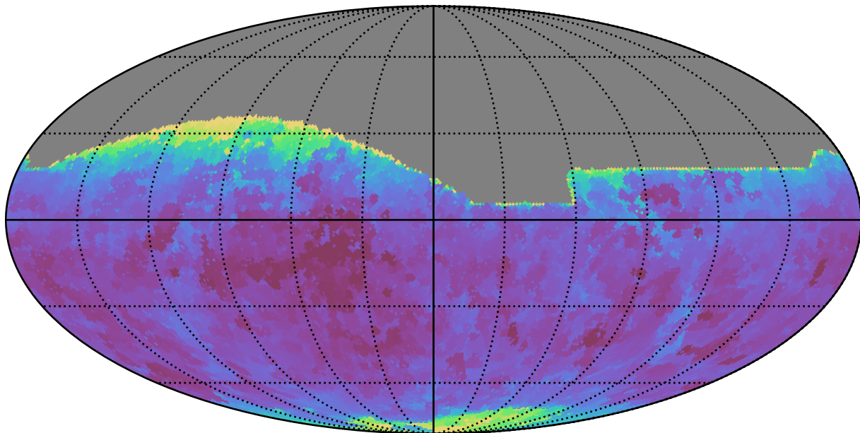
baseline_v3.3_10yrs All sky r band: Min seeingEff
