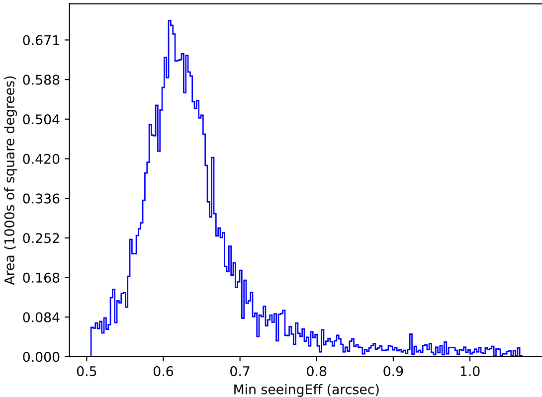
baseline_v3.3_10yrs All sky r band: Min seeingEff
