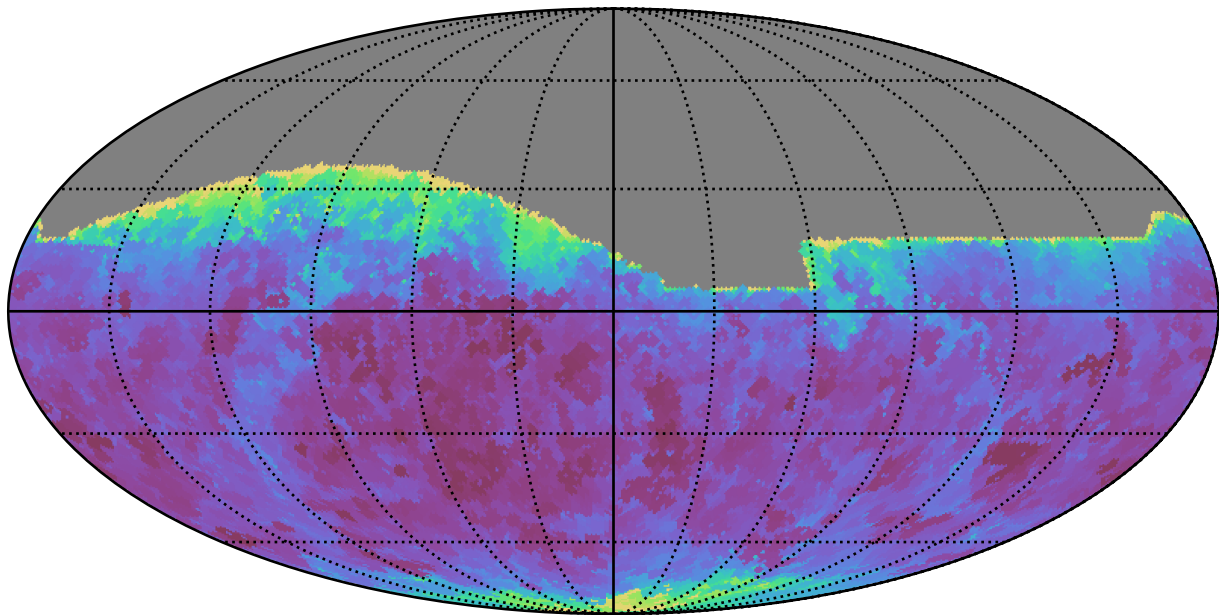
baseline_v3.3_10yrs All sky i band: Min seeingEff
