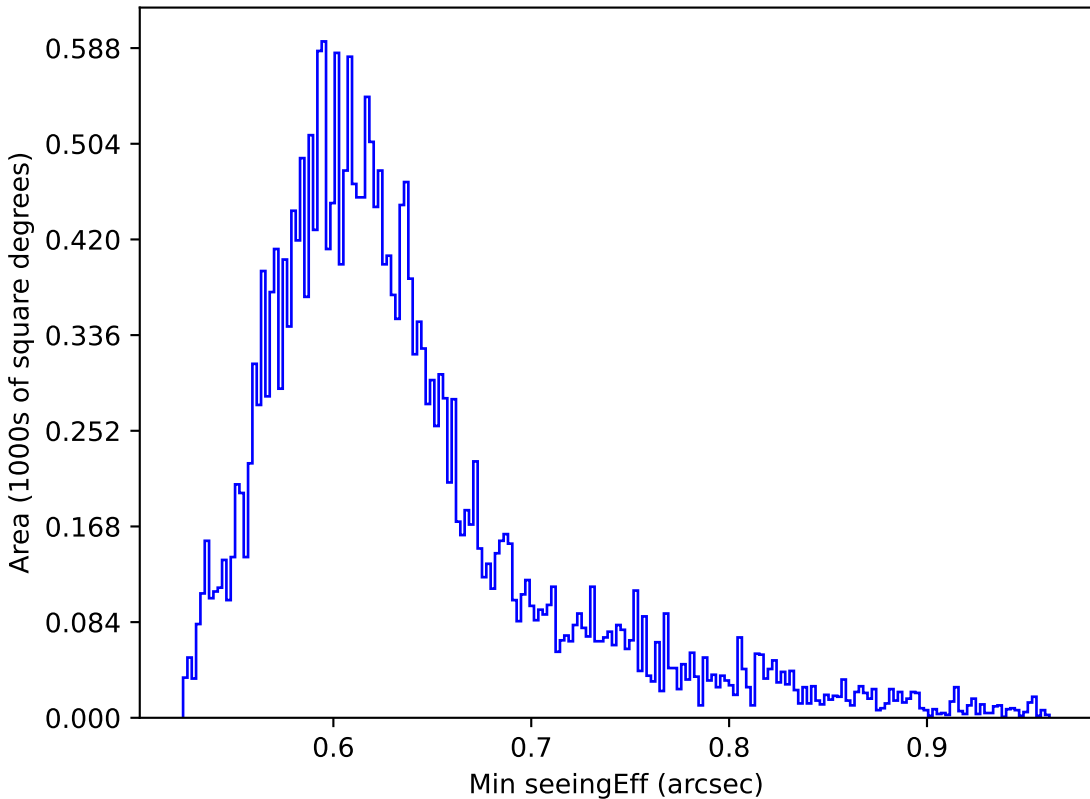
baseline_v3.3_10yrs All sky i band: Min seeingEff
