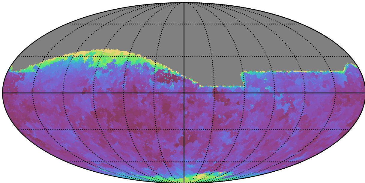
baseline_v3.3_10yrs All sky g band: Min seeingEff
