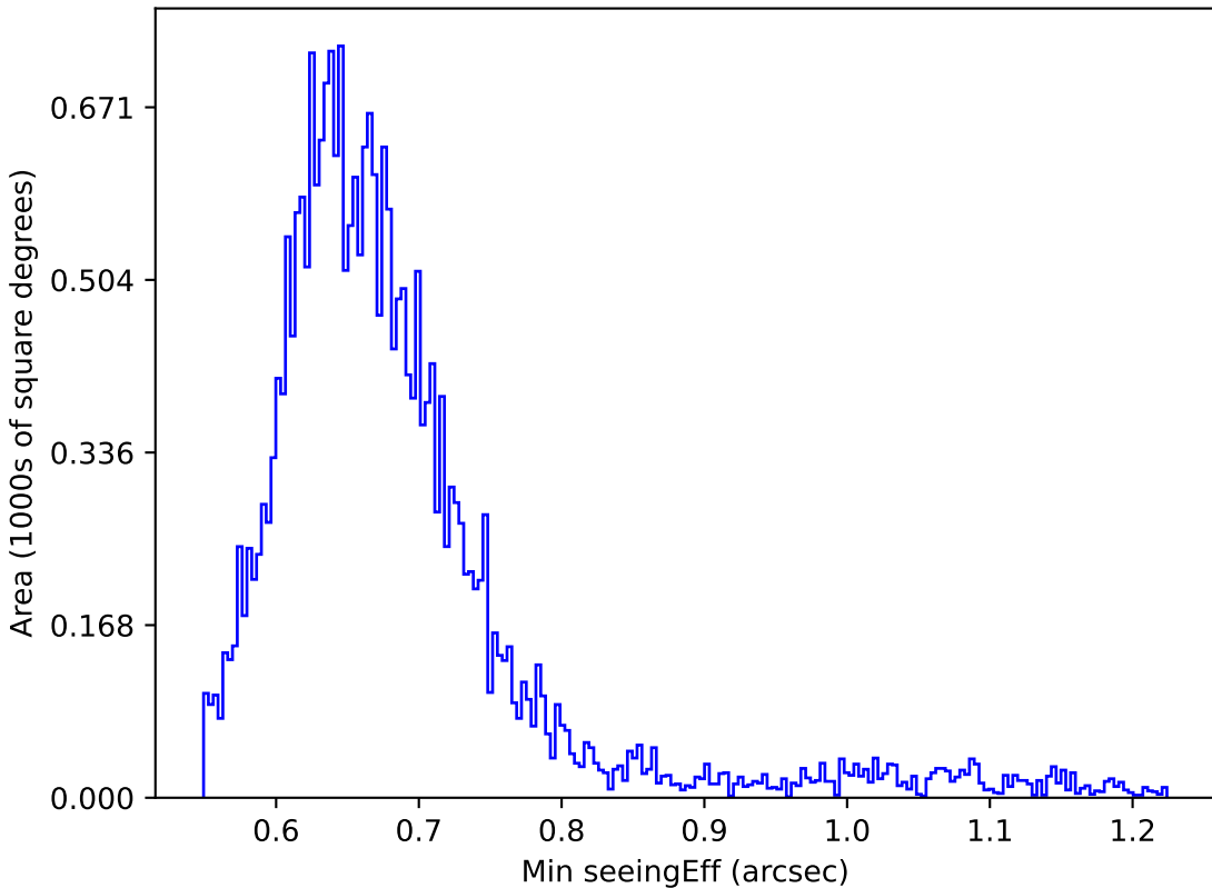
baseline_v3.3_10yrs All sky g band: Min seeingEff
