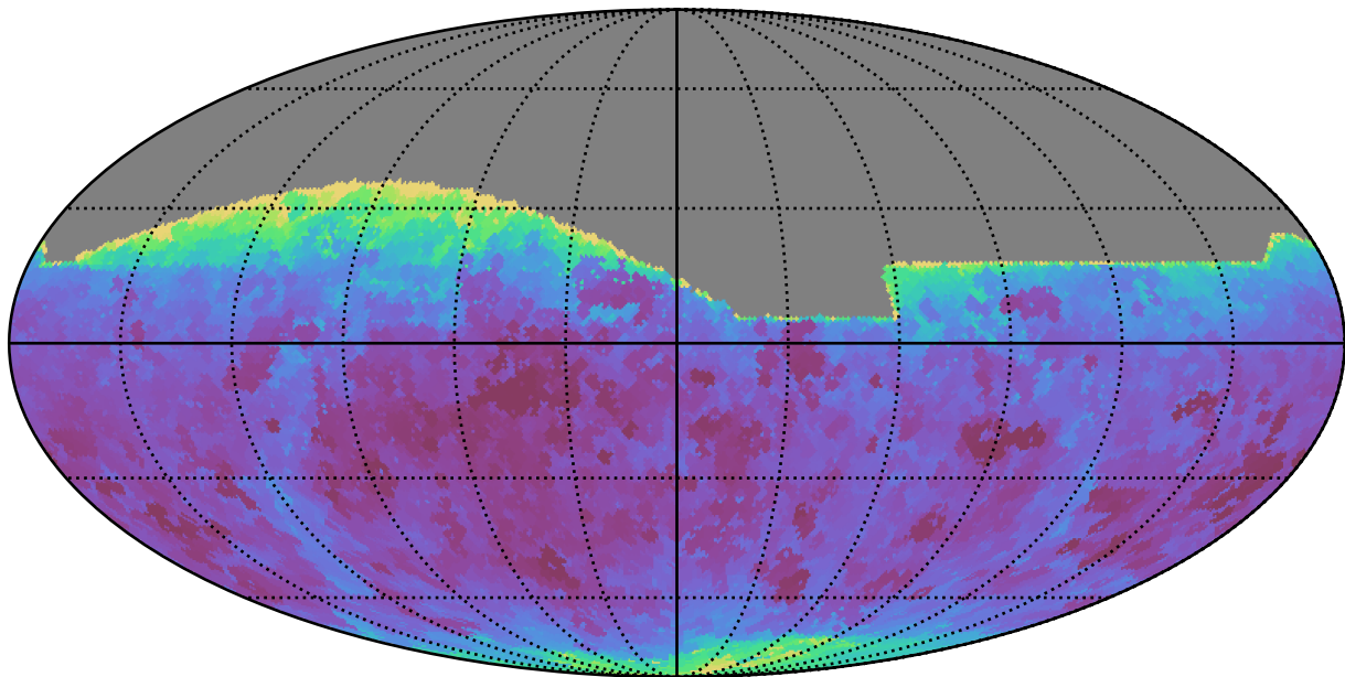
baseline_v3.3_10yrs All sky all bands: Min seeingEff
