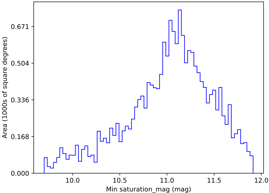
baseline_v3.3_10yrs WFD all bands: Min saturation_mag
