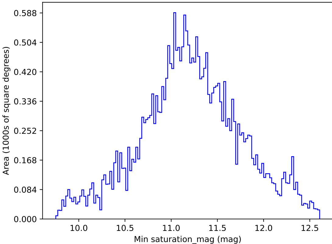
baseline_v3.3_10yrs All sky all bands: Min saturation_mag
