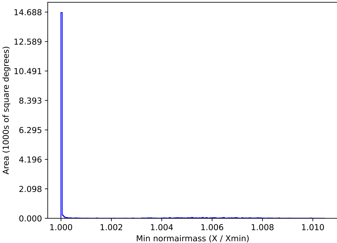
baseline_v3.3_10yrs WFD all bands: Min normairmass
