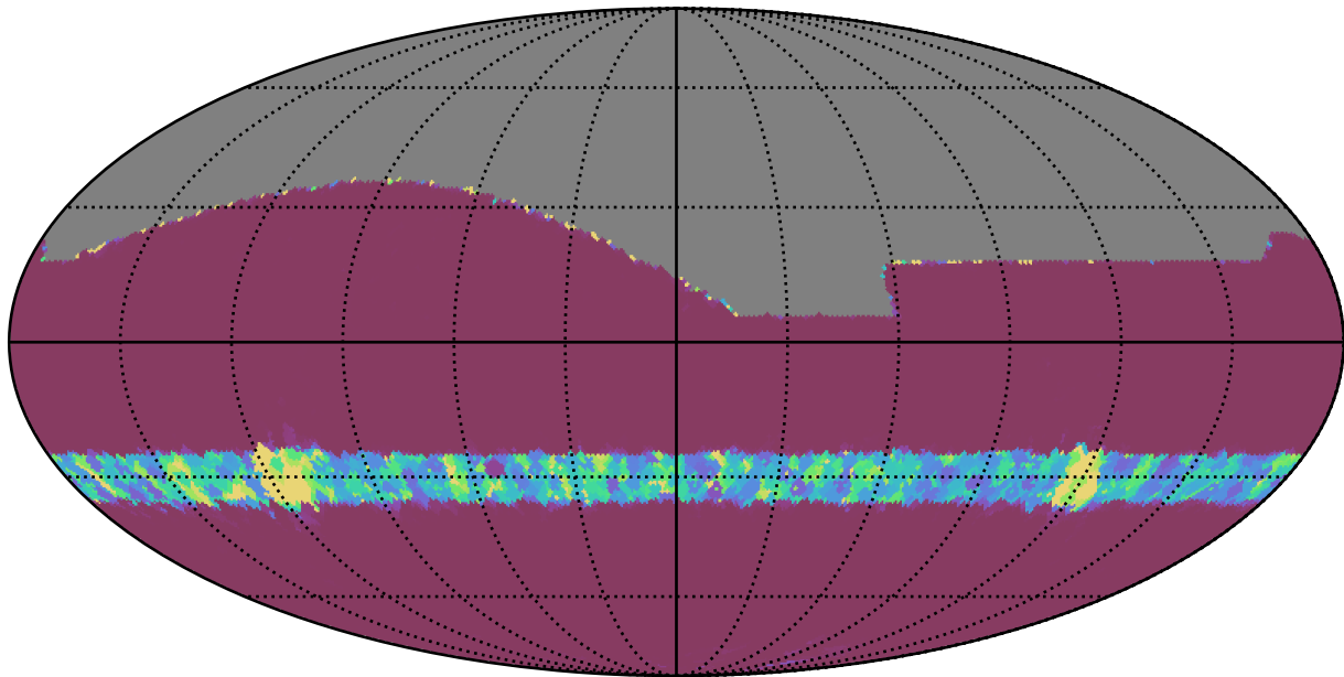
baseline_v3.3_10yrs All sky all bands: Min normairmass
