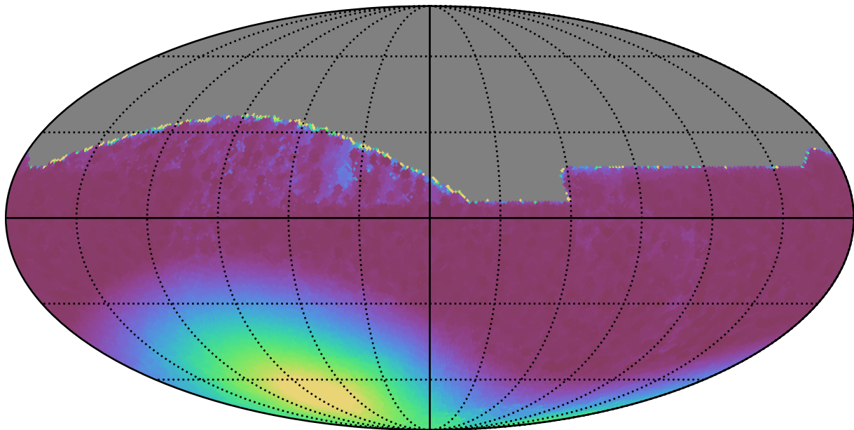
baseline_v3.3_10yrs All sky all bands: Min moonDistance
