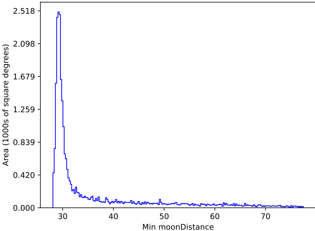
baseline_v3.3_10yrs All sky all bands: Min moonDistance
