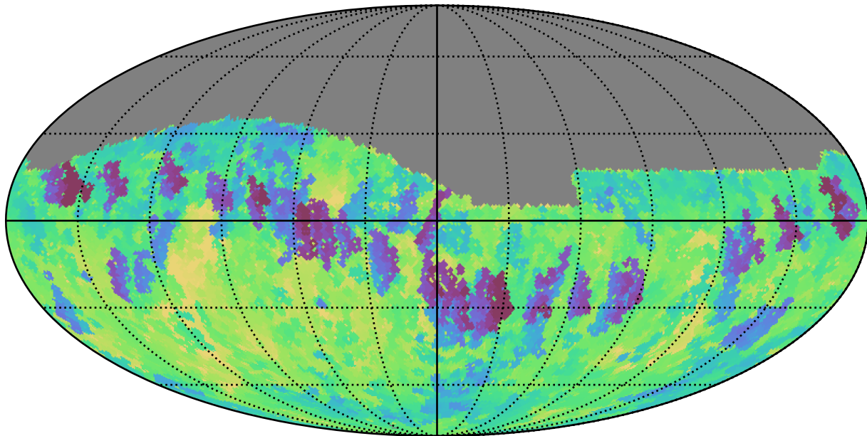
baseline_v3.3_10yrs Yr 1 z band: Min fiveSigmaDepth
