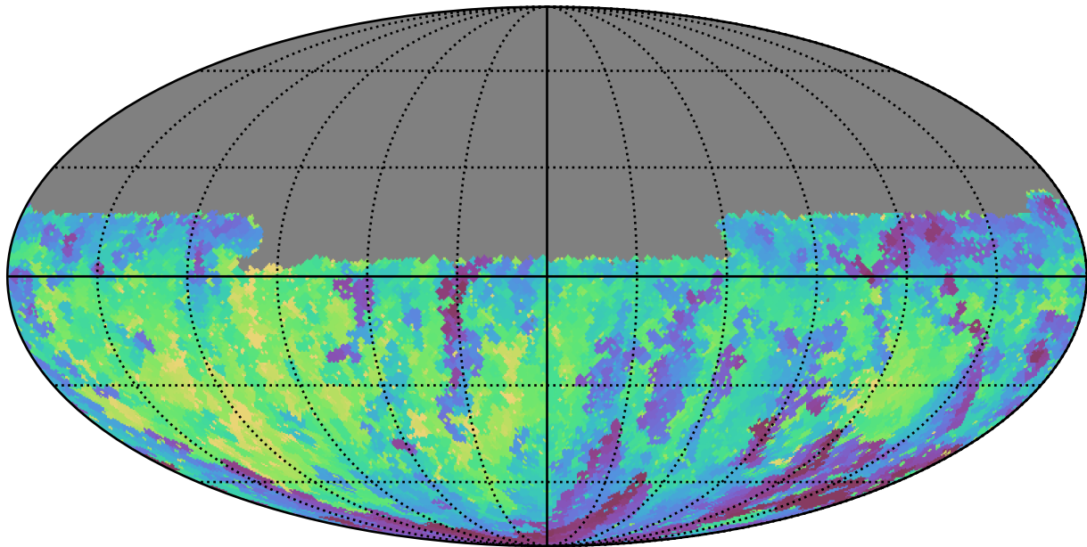
baseline_v3.3_10yrs Yr 1 u band: Min fiveSigmaDepth
