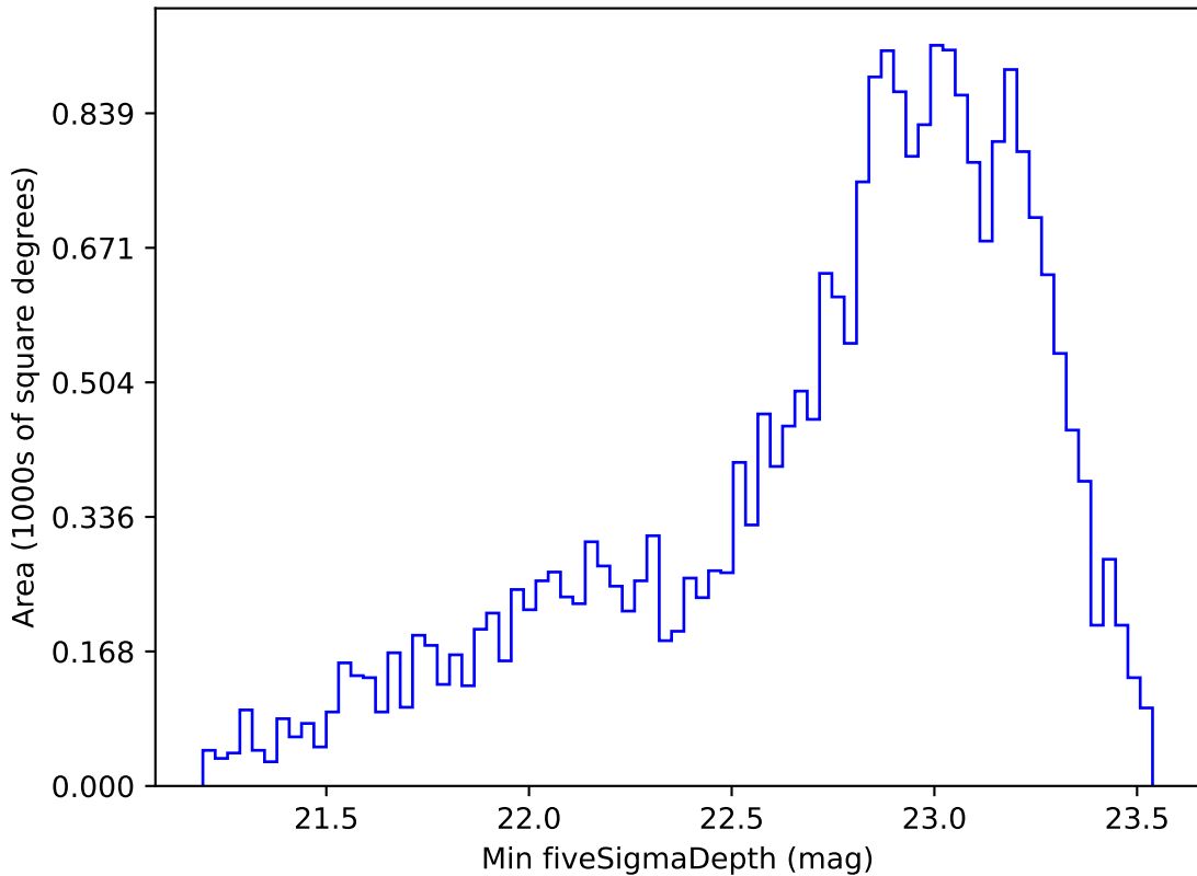
baseline_v3.3_10yrs Yr 1 i band: Min fiveSigmaDepth
