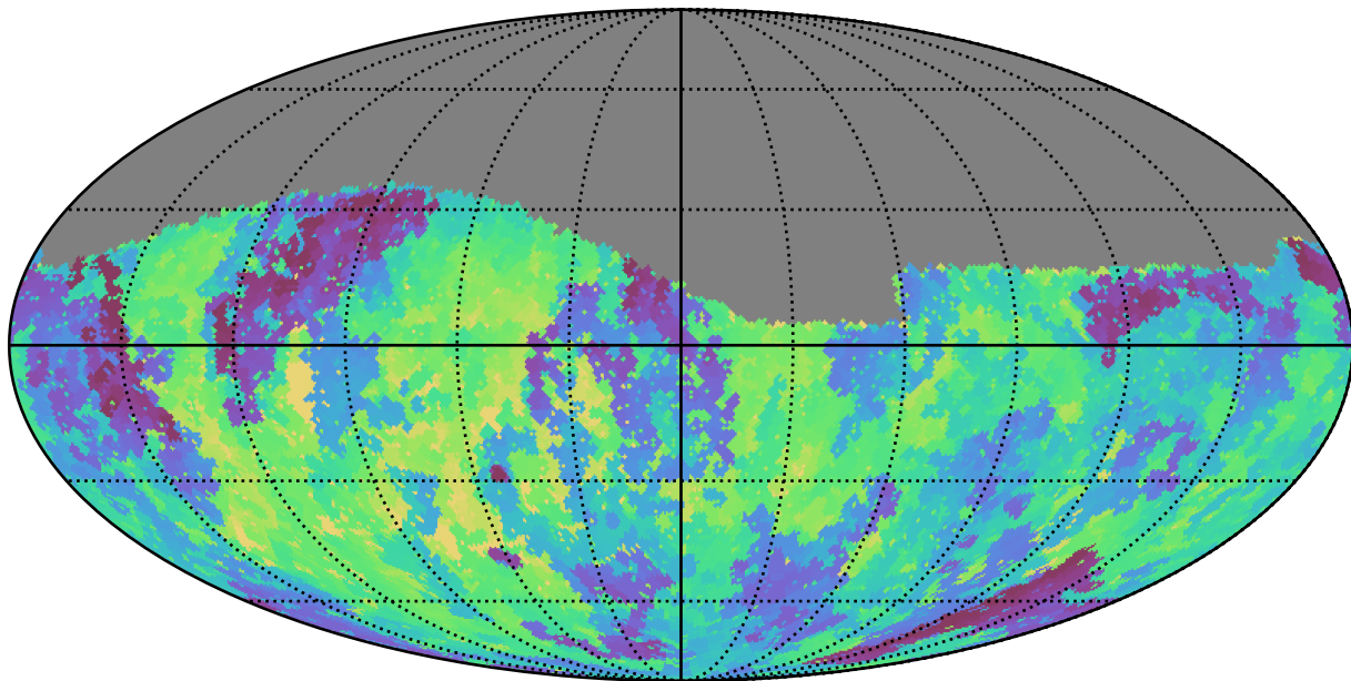
baseline_v3.3_10yrs Yr 1 g band: Min fiveSigmaDepth
