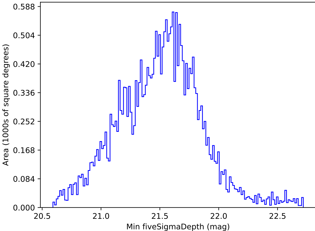
baseline_v3.3_10yrs Yr 1 all bands: Min fiveSigmaDepth
