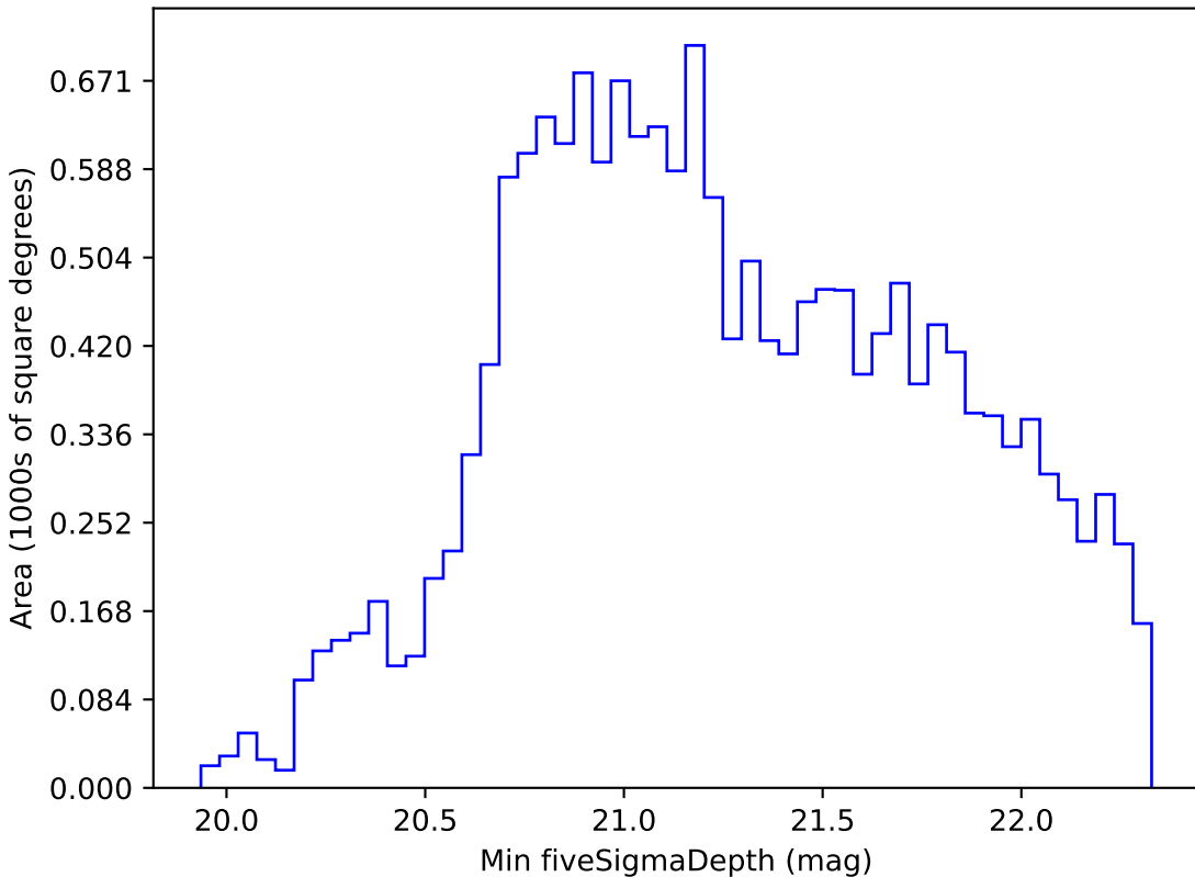
baseline_v3.3_10yrs WFD z band: Min fiveSigmaDepth
