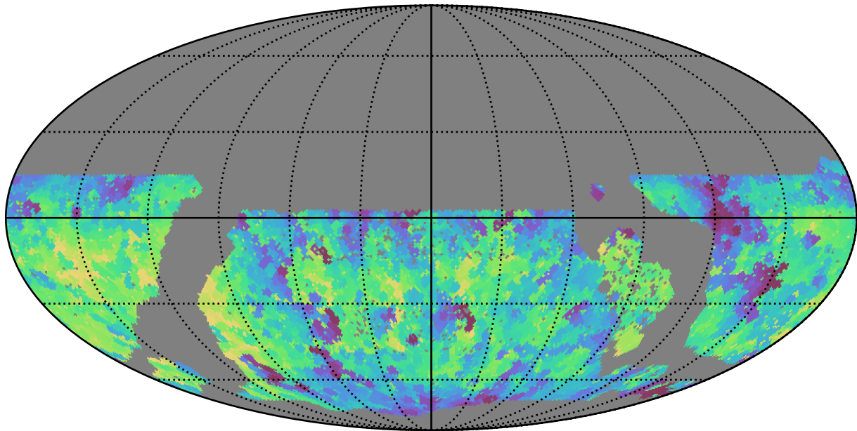
baseline_v3.3_10yrs WFD u band: Min fiveSigmaDepth
