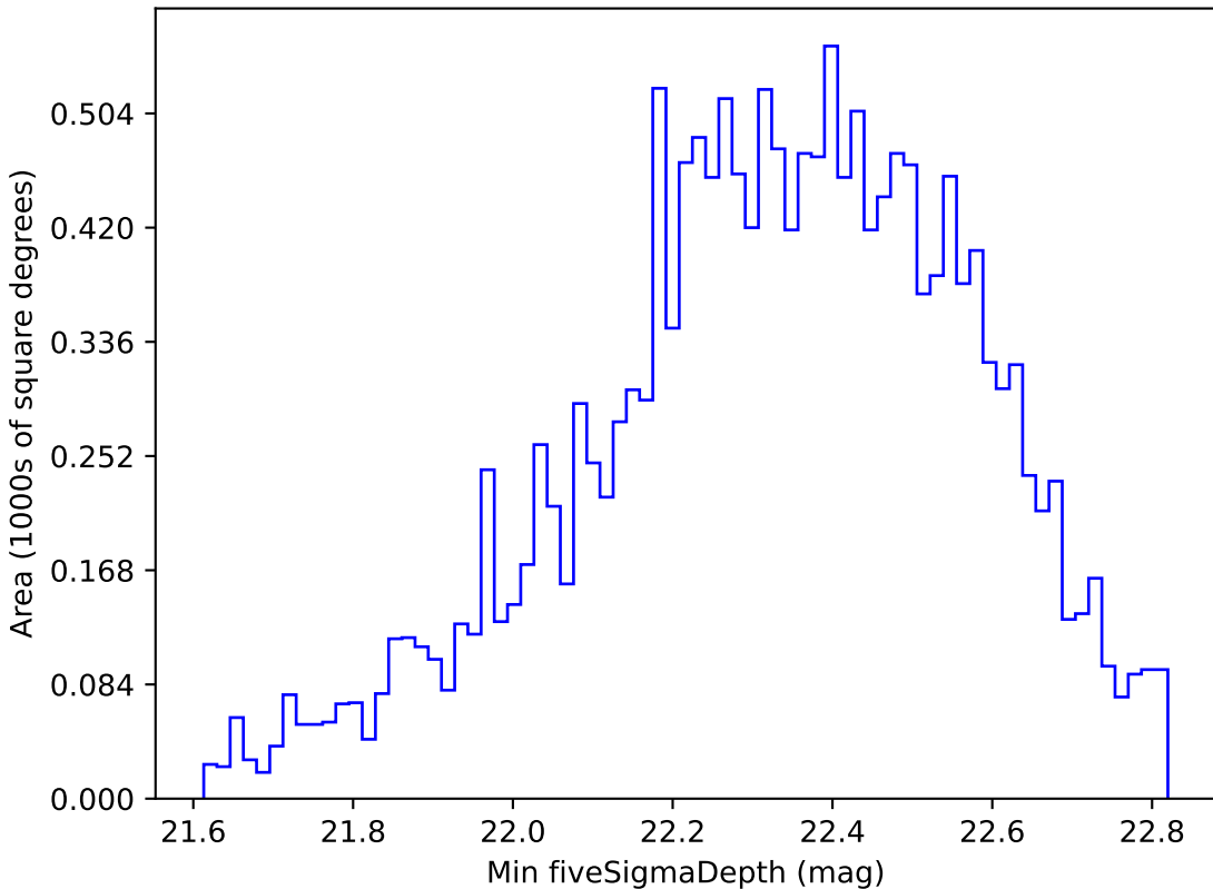
baseline_v3.3_10yrs WFD u band: Min fiveSigmaDepth
