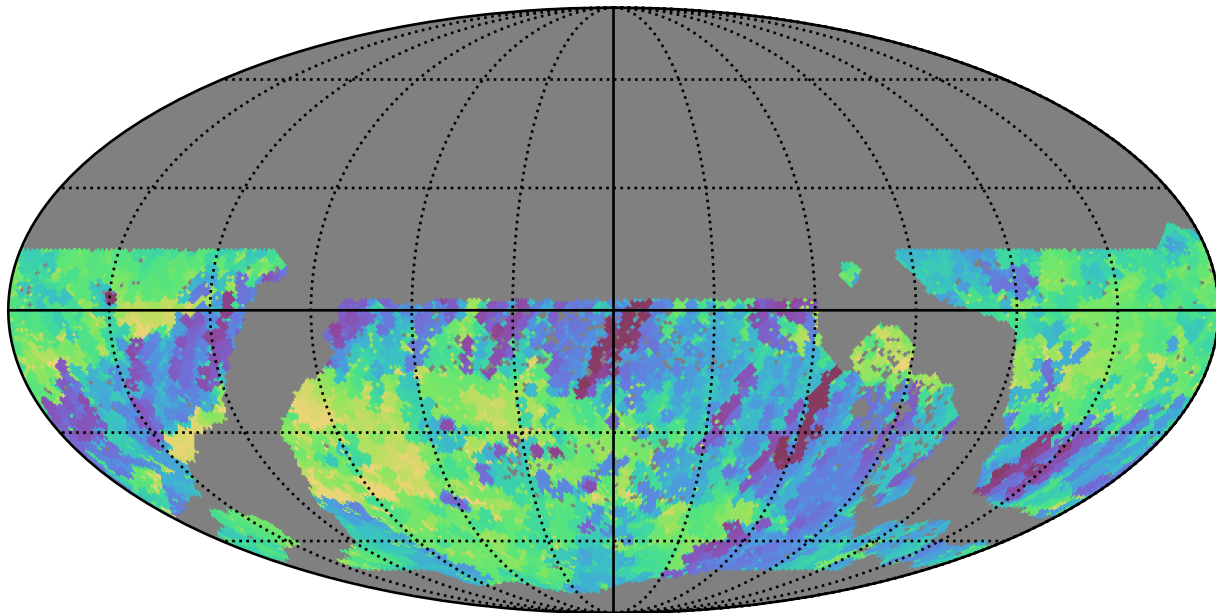
baseline_v3.3_10yrs WFD r band: Min fiveSigmaDepth
