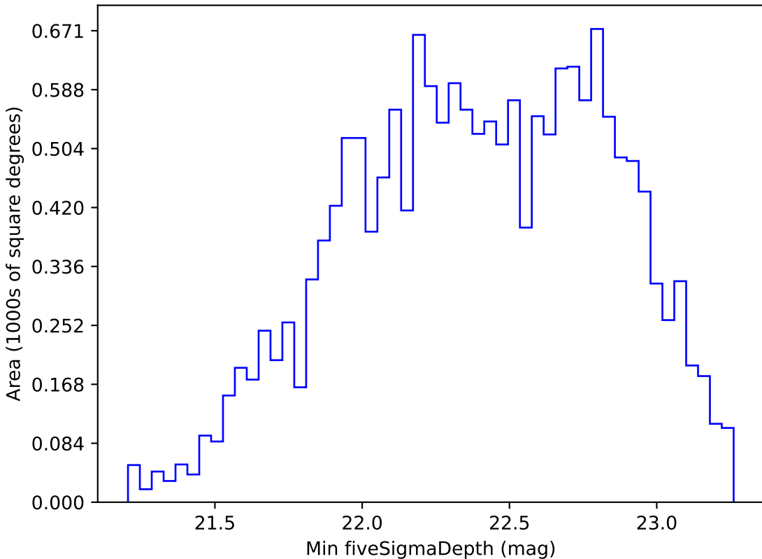
baseline_v3.3_10yrs WFD r band: Min fiveSigmaDepth
