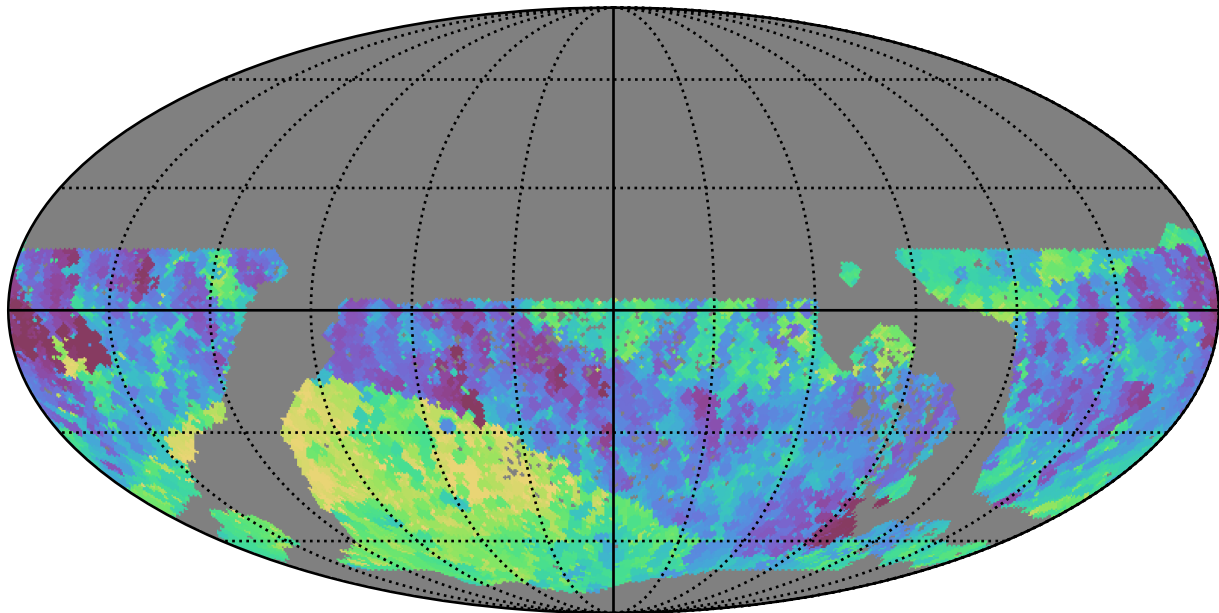
baseline_v3.3_10yrs WFD i band: Min fiveSigmaDepth
