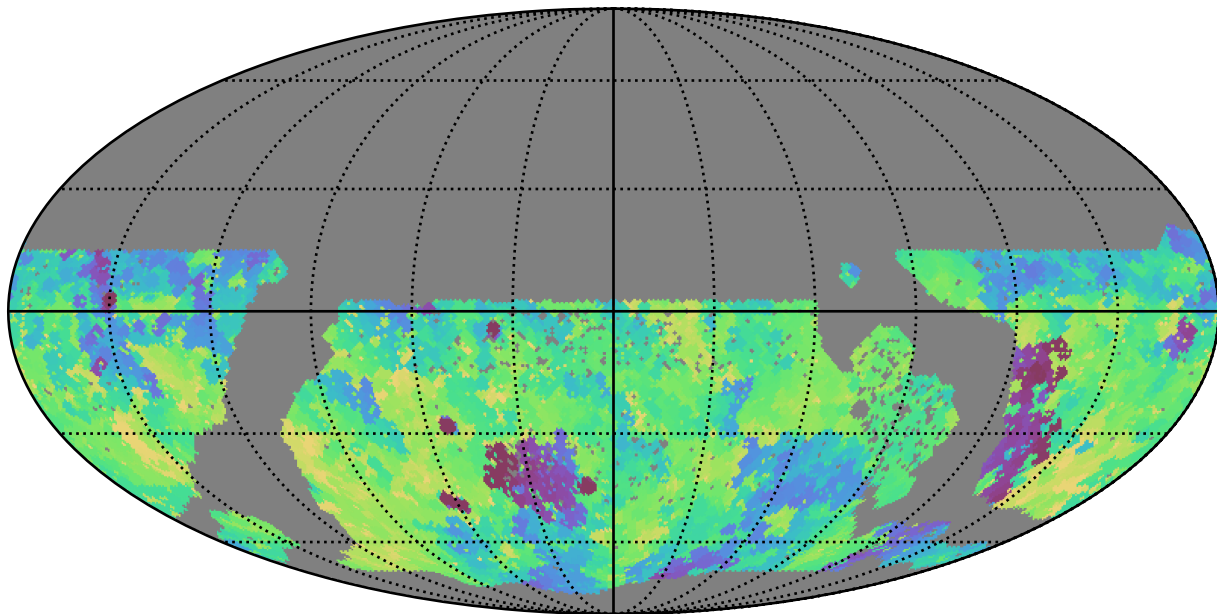
baseline_v3.3_10yrs WFD g band: Min fiveSigmaDepth
