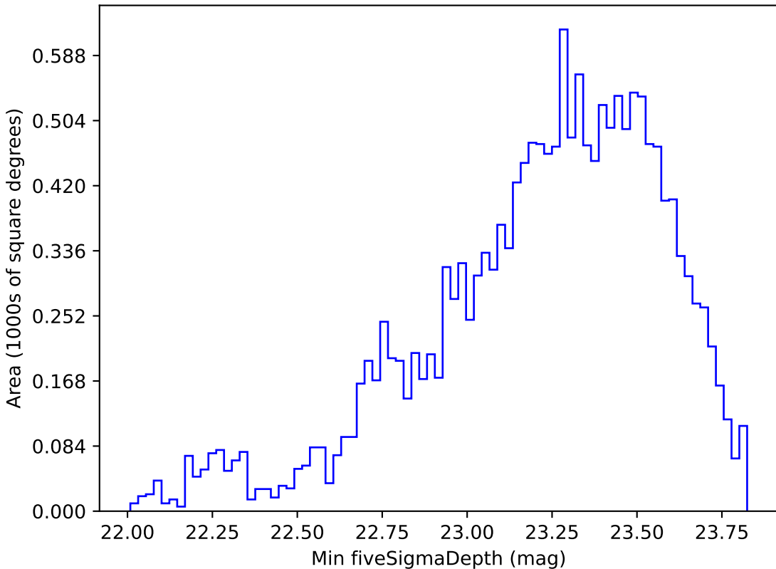
baseline_v3.3_10yrs WFD g band: Min fiveSigmaDepth
