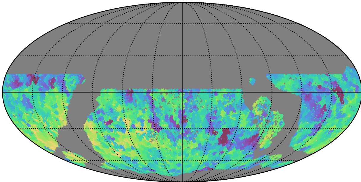
baseline_v3.3_10yrs WFD all bands: Min fiveSigmaDepth
