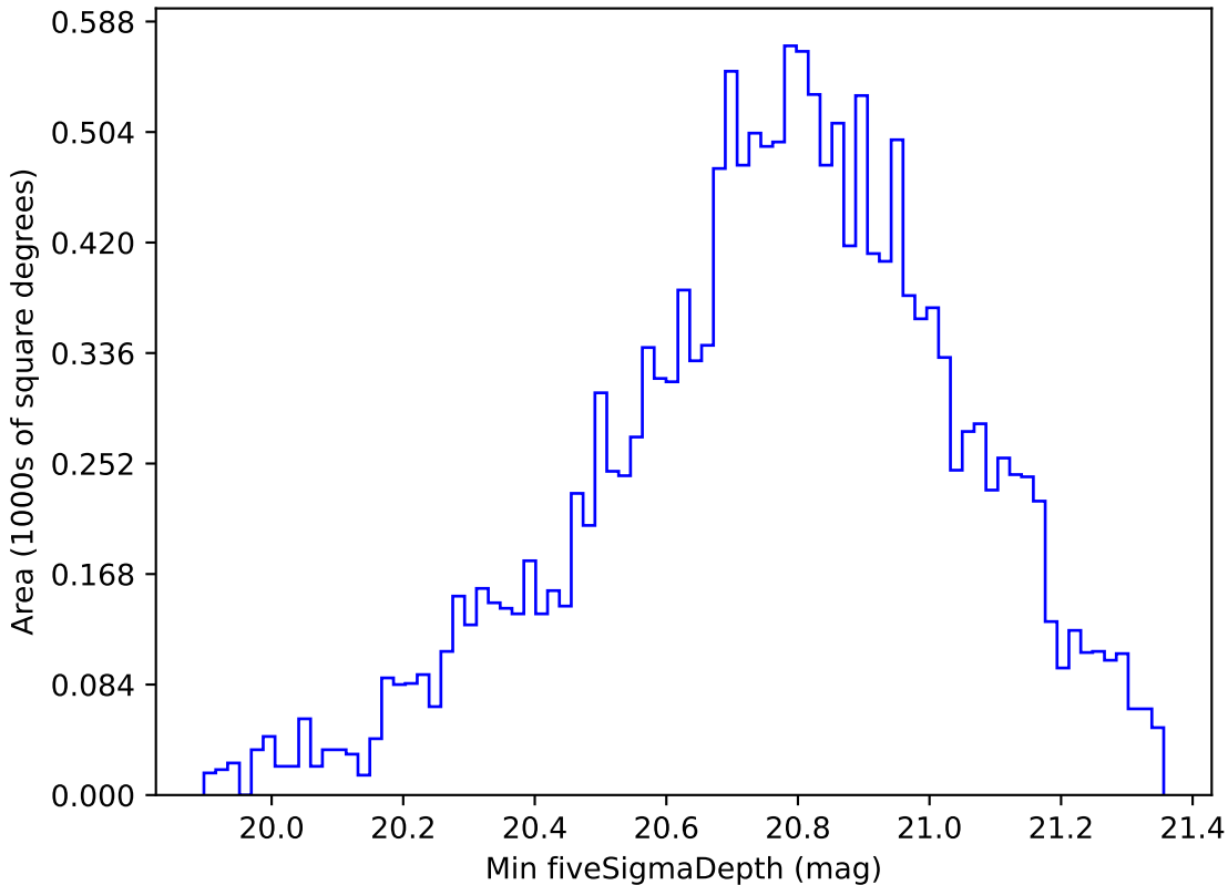
baseline_v3.3_10yrs WFD all bands: Min fiveSigmaDepth
