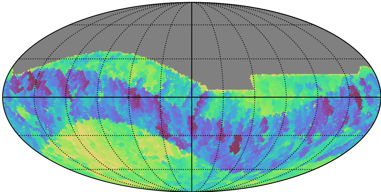
baseline_v3.3_10yrs All sky z band: Min fiveSigmaDepth
