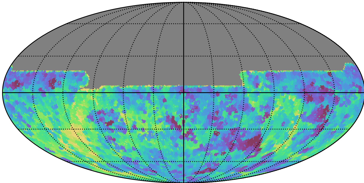
baseline_v3.3_10yrs All sky y band: Min fiveSigmaDepth
