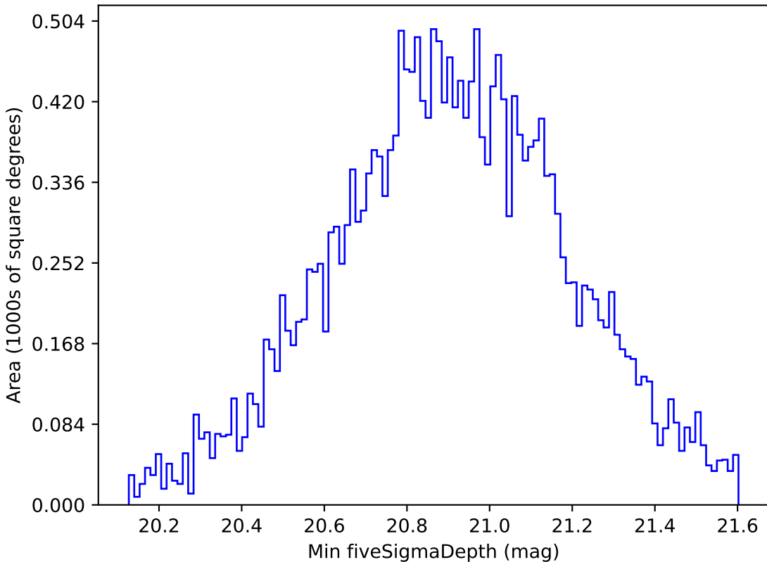
baseline_v3.3_10yrs All sky y band: Min fiveSigmaDepth
