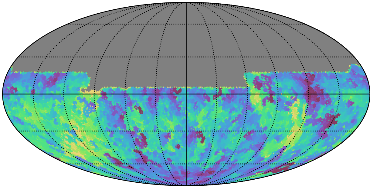
baseline_v3.3_10yrs All sky u band: Min fiveSigmaDepth
