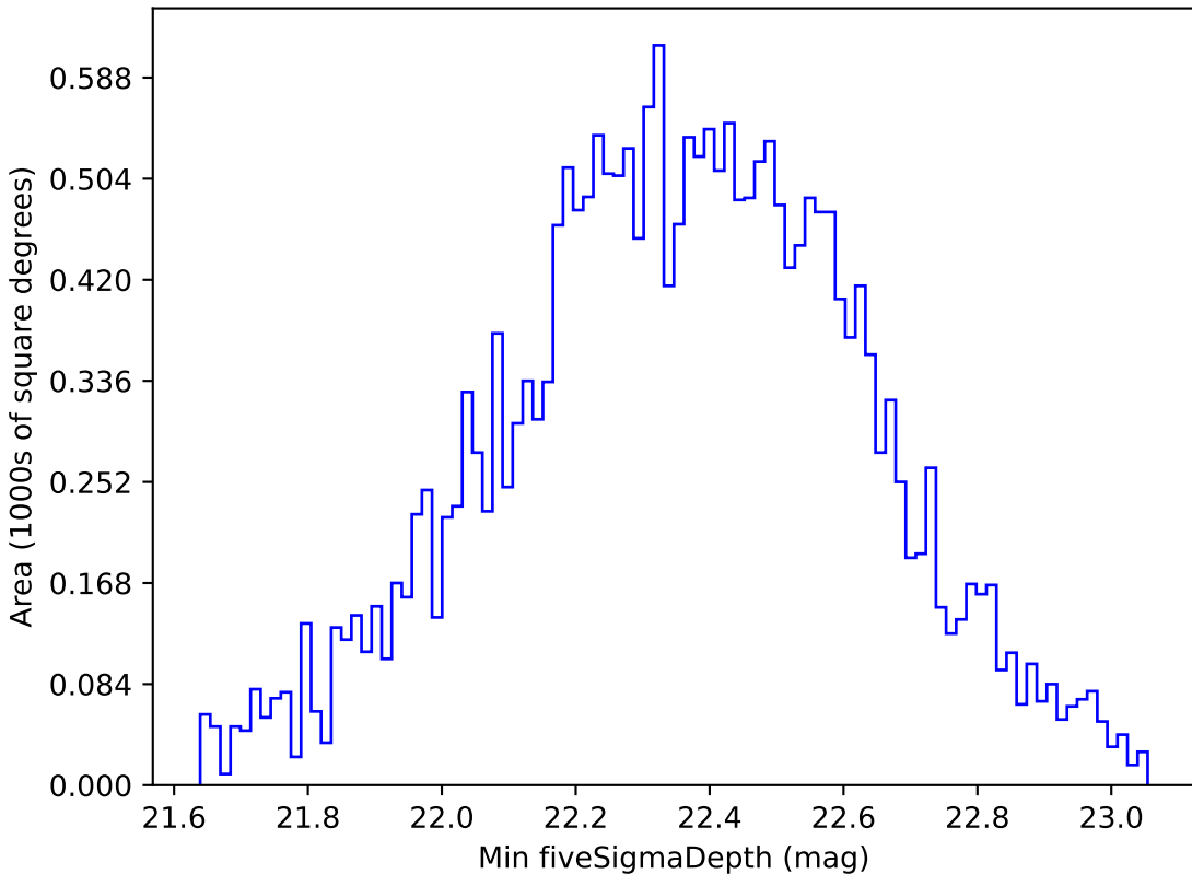
baseline_v3.3_10yrs All sky u band: Min fiveSigmaDepth
