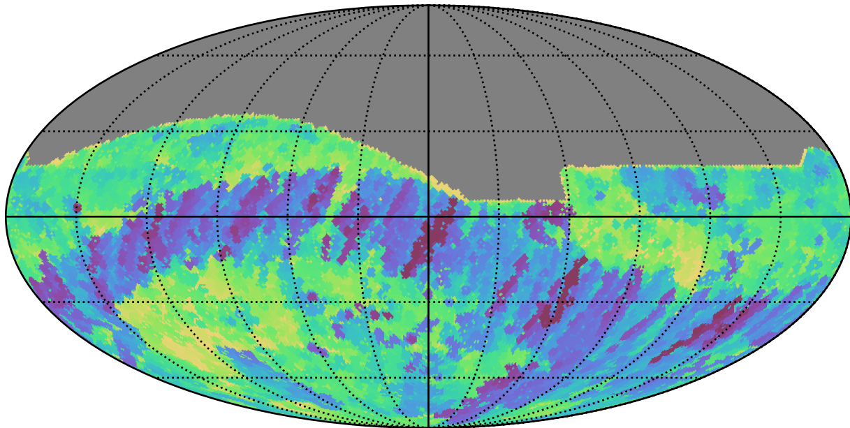
baseline_v3.3_10yrs All sky r band: Min fiveSigmaDepth
