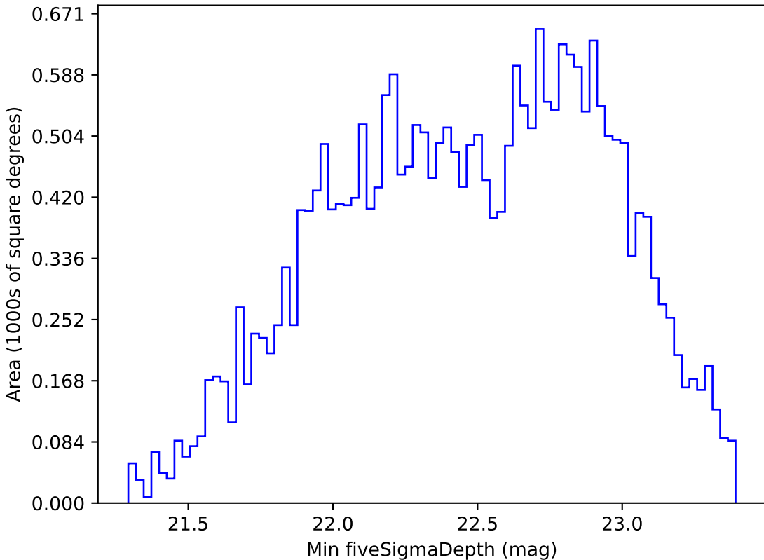
baseline_v3.3_10yrs All sky r band: Min fiveSigmaDepth
