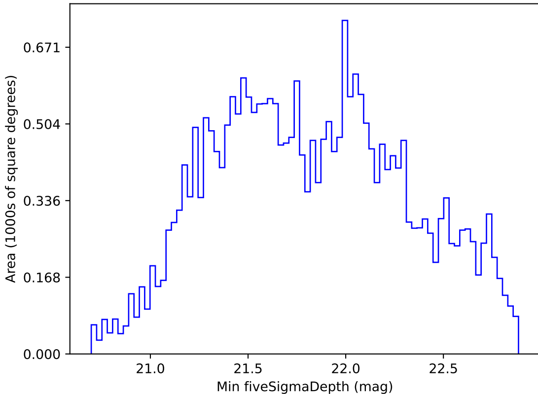
baseline_v3.3_10yrs All sky i band: Min fiveSigmaDepth
