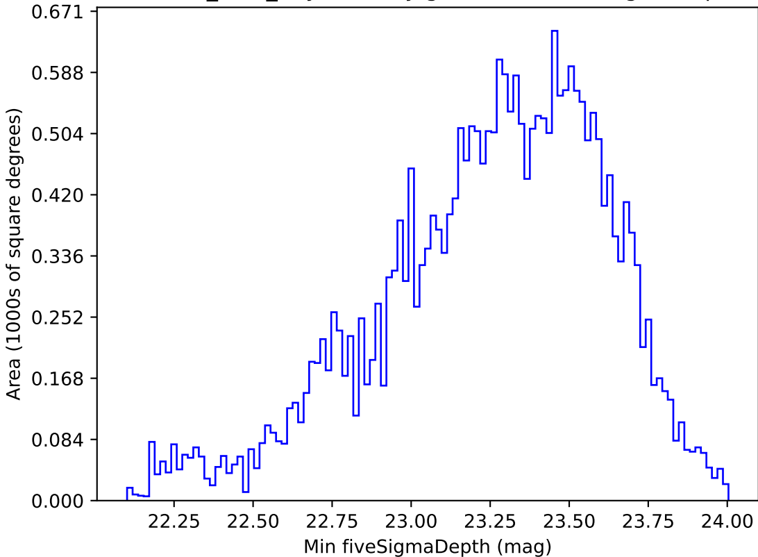
baseline_v3.3_10yrs All sky g band: Min fiveSigmaDepth
