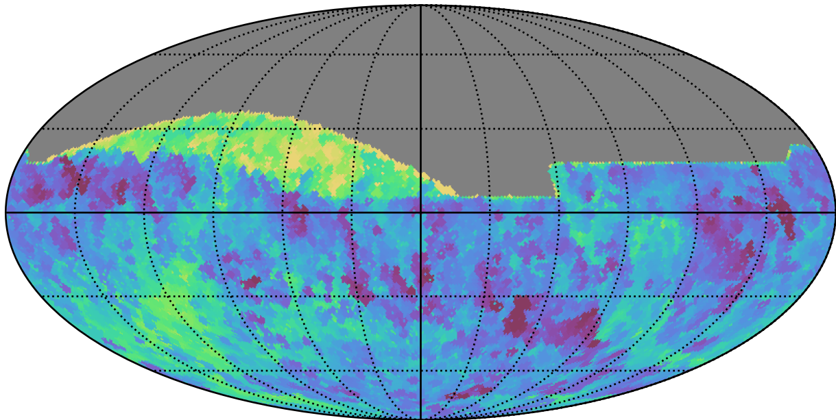
baseline_v3.3_10yrs All sky all bands: Min fiveSigmaDepth
