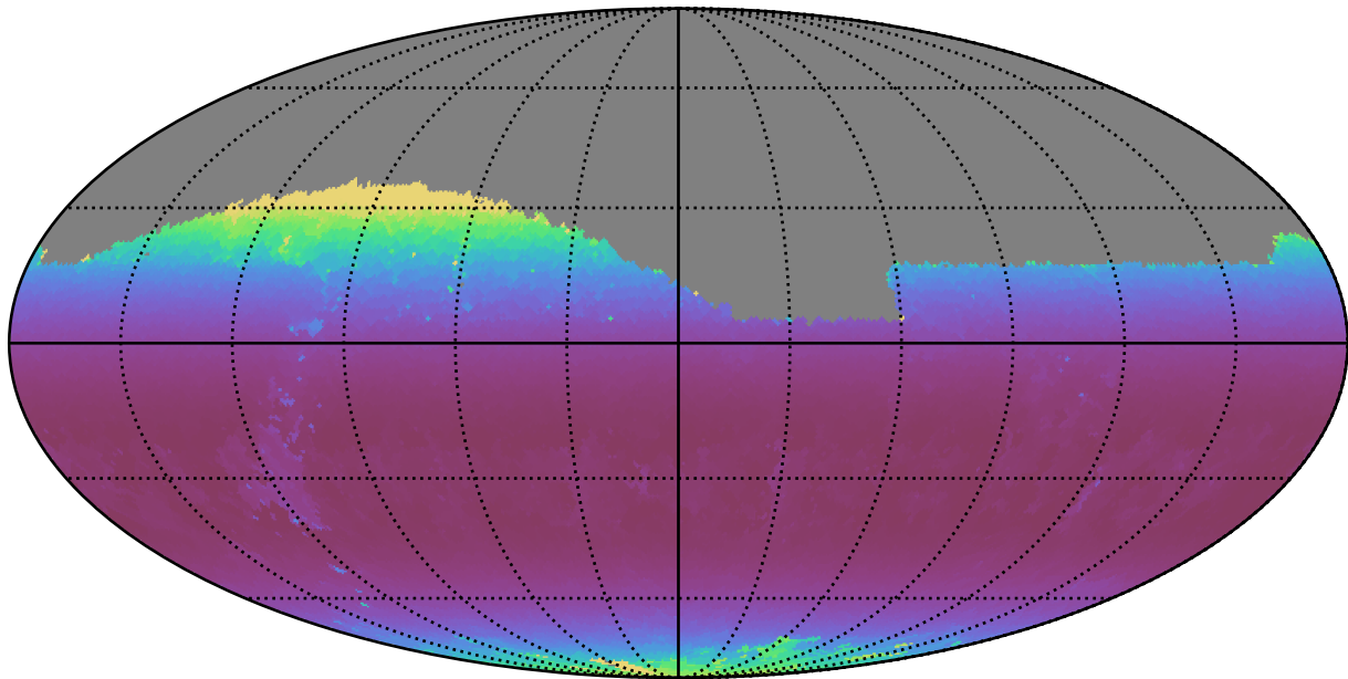
baseline_v3.3_10yrs Yr 1 z band: Min airmass
