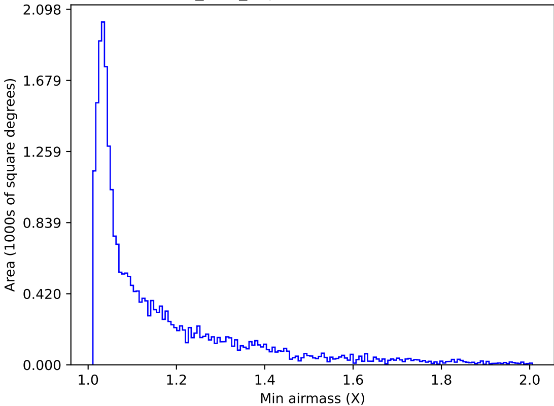
baseline_v3.3_10yrs Yr 1 z band: Min airmass
