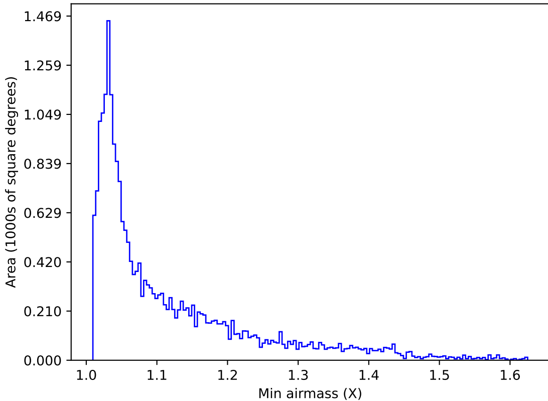
baseline_v3.3_10yrs Yr 1 y band: Min airmass
