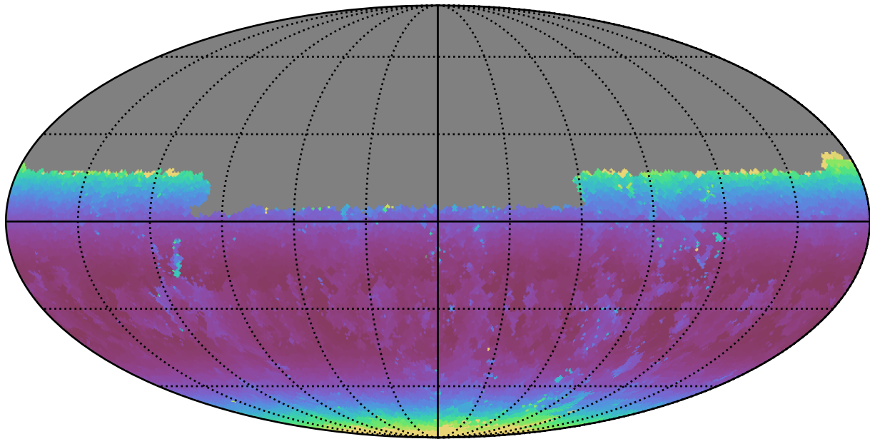
baseline_v3.3_10yrs Yr 1 u band: Min airmass
