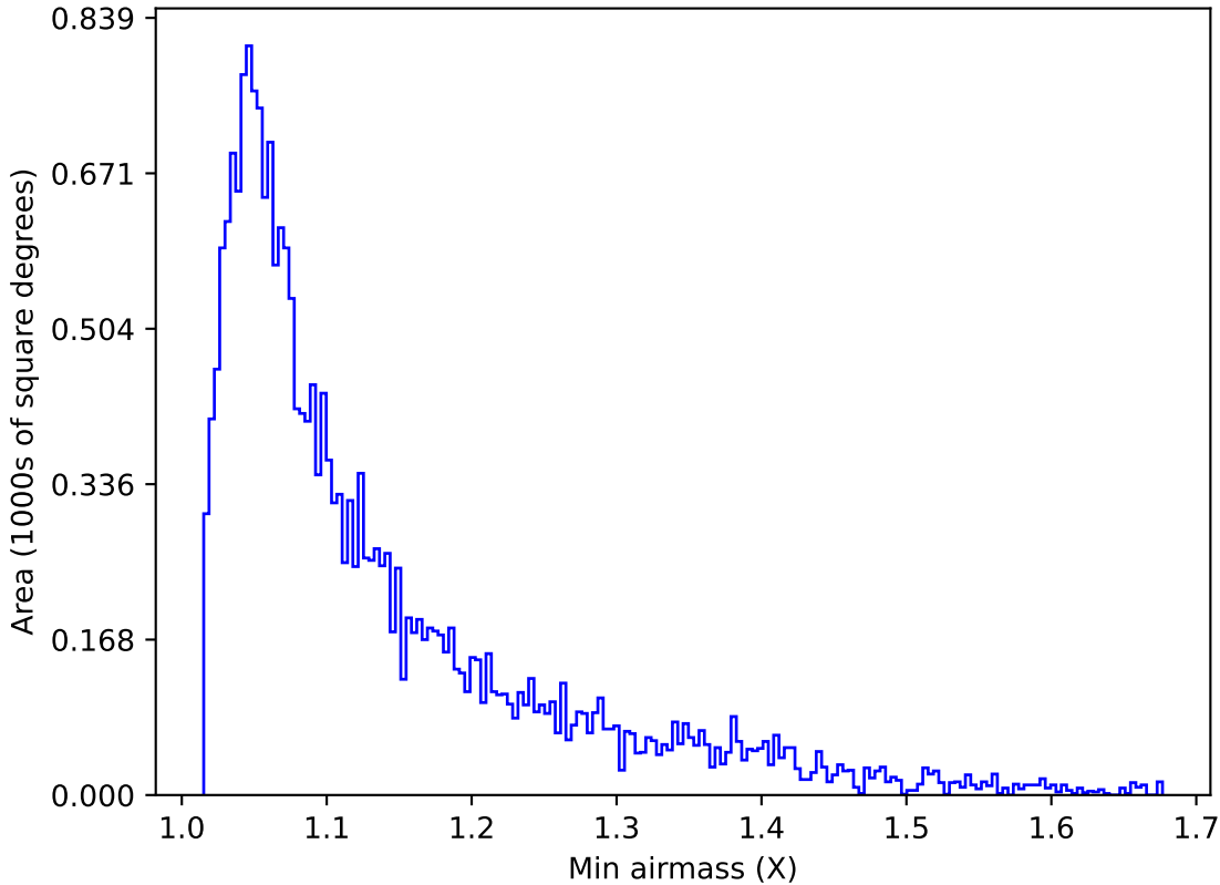
baseline_v3.3_10yrs Yr 1 u band: Min airmass
