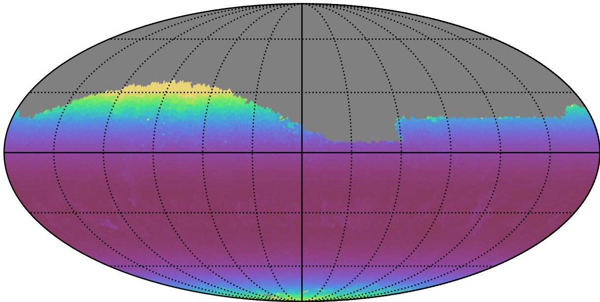
baseline_v3.3_10yrs Yr 1 r band: Min airmass
