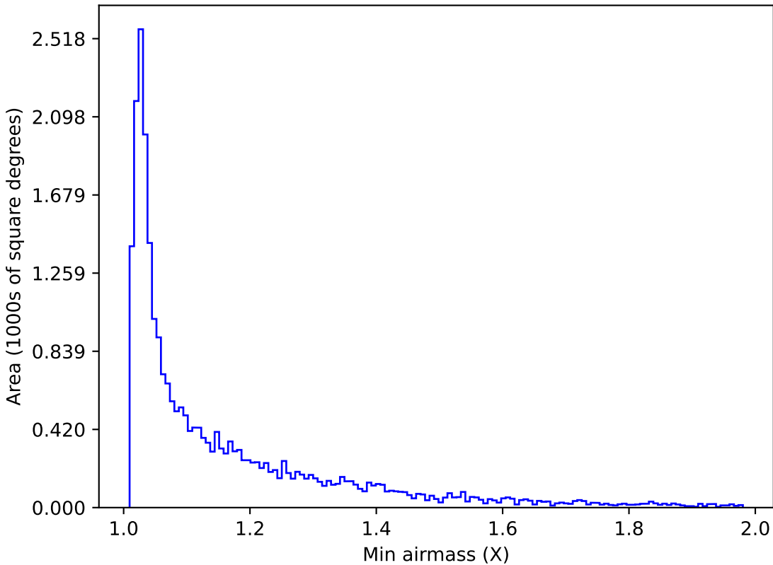
baseline_v3.3_10yrs Yr 1 r band: Min airmass
