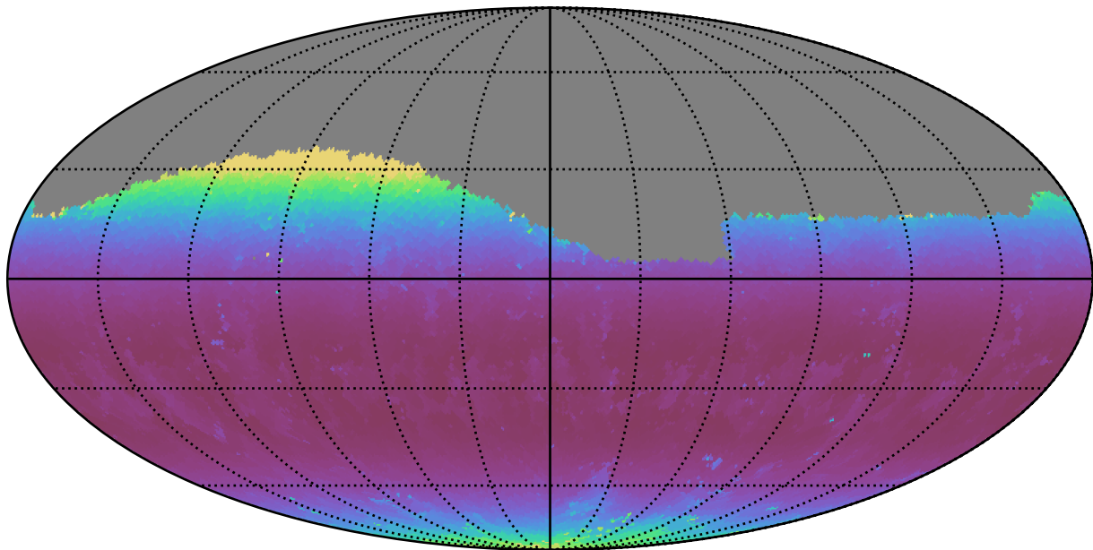
baseline_v3.3_10yrs Yr 1 g band: Min airmass
