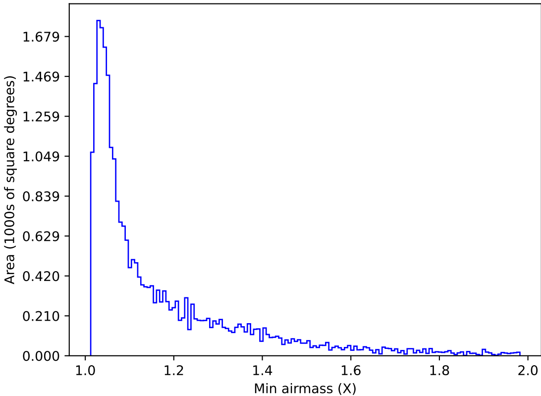
baseline_v3.3_10yrs Yr 1 g band: Min airmass
